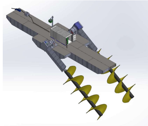
Tidal Platform by Jupiter Hydro Inc that can be mounted on a fixed or floating platform
